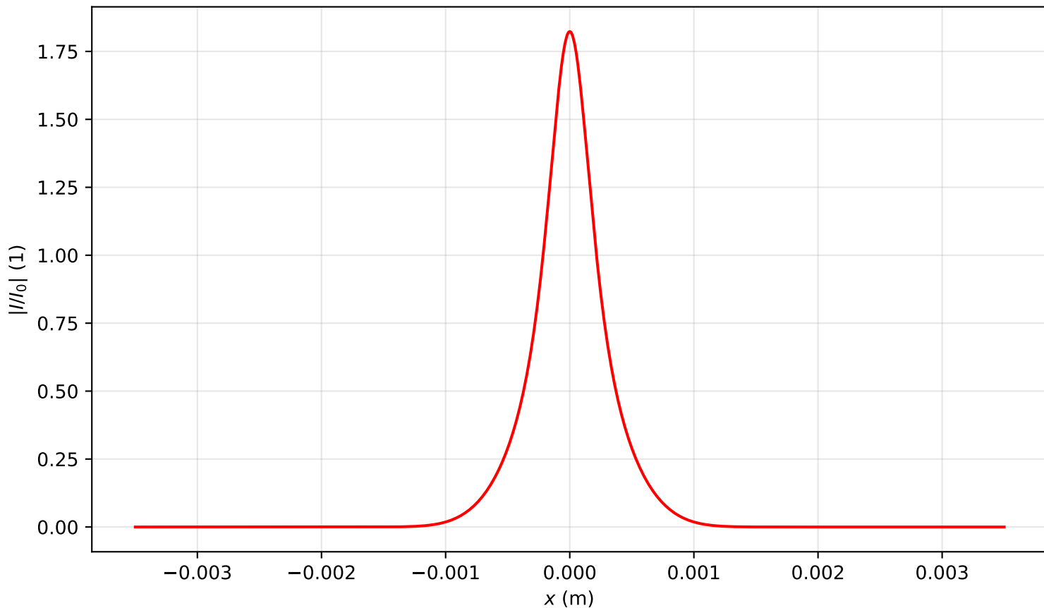
Intensity profile I(x, y = 0, z = 0.478)/I_0 , P_{in}=2.5P_{cr} , artificial time
